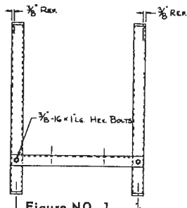
Figure NO. 1 Assembly Detail of Stand
