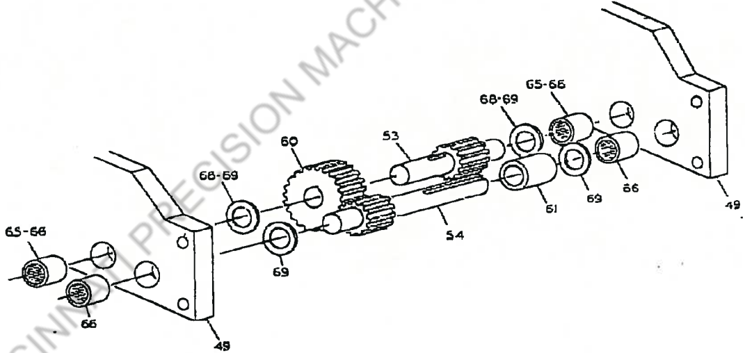
FIRST 2 PINIONS OF 4 PINION REDUCER
