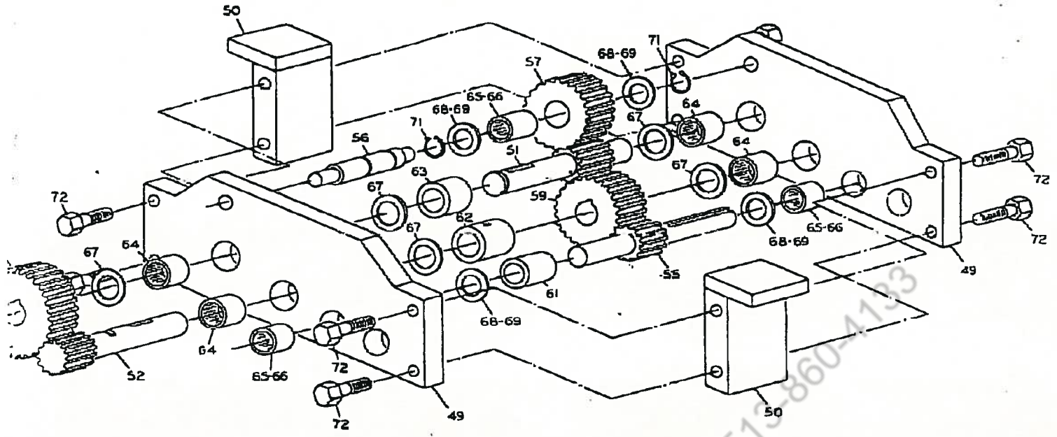
3 PINION REDUCER
